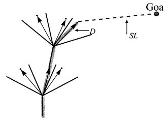
Fig. 5. Node is expanded only if D + SL \leq d-max .
