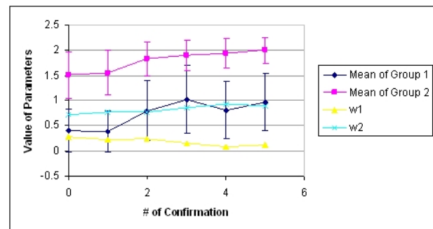
Fig. 4. Parameters for the density function, fitting p(x) = w_1p_1(x) + w_2p_2(x) for the metric of support for PPI data with different confirmation numbers. Group 1 corresponds to noise, and Group 2 to signal.
