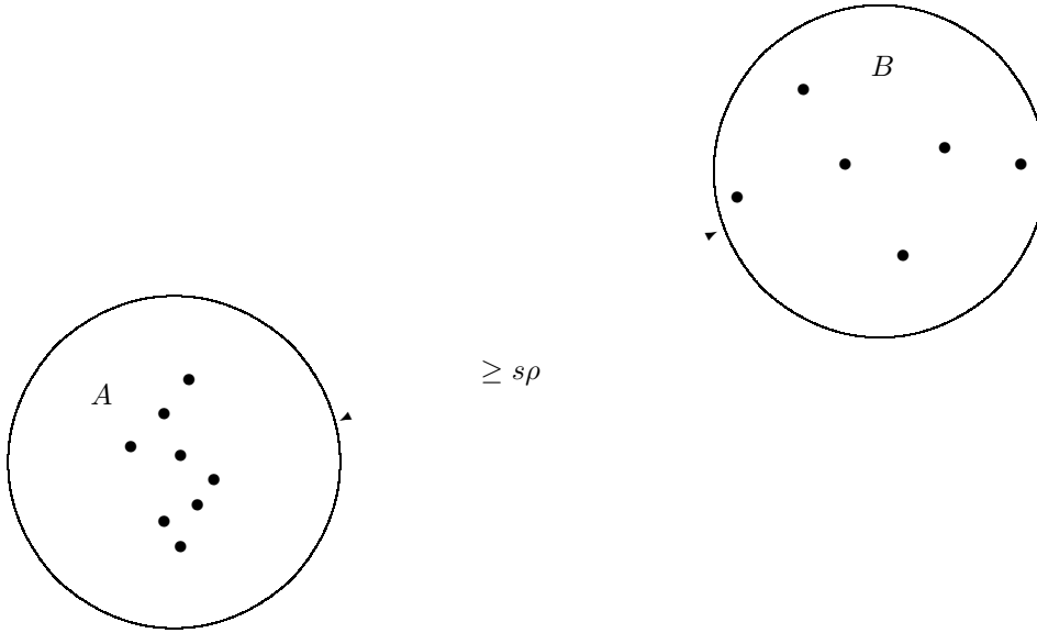
FIG. 2.1. Two planar point sets A and B that are well-separated w.r.t. s . Both circles have radius \rho ; their distance is at least s\rho .
