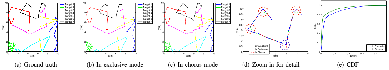
Fig. 14. Tracking fidelity contrast between chorus mode and exclusive mode
