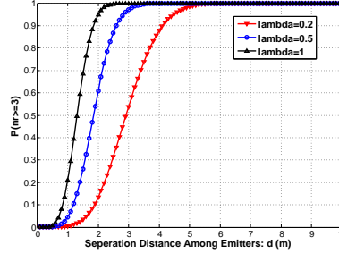
Fig. 7. Probability of three receivers are in TDR
