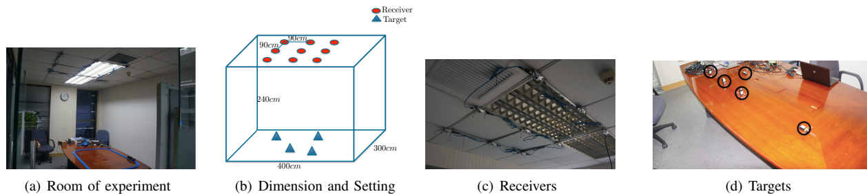
Fig. 16. Setting of test-bed
