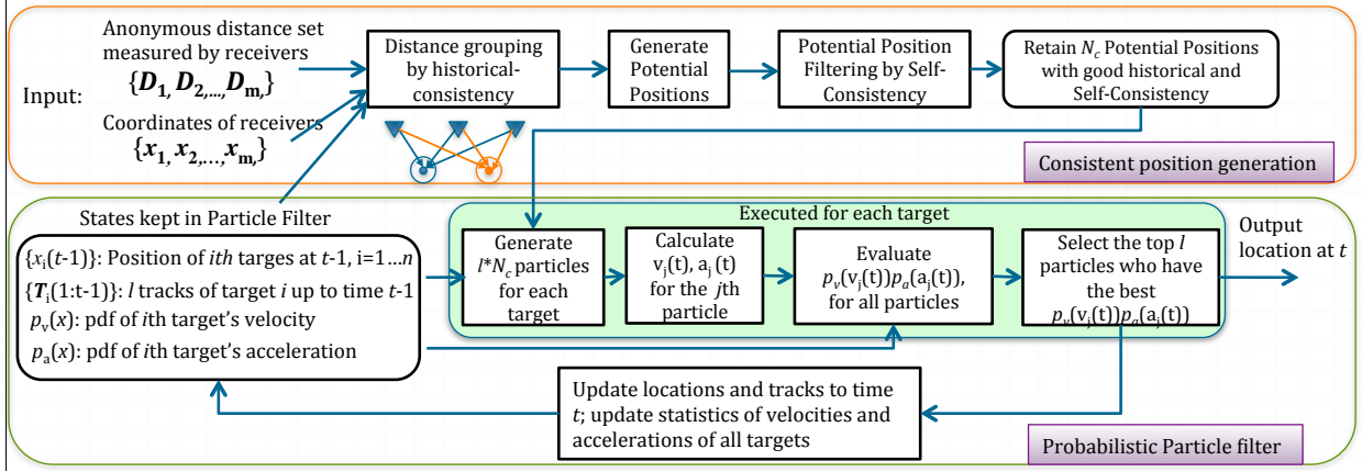
Fig. 9. The diagram of consistent location generation and probabilistic particle filter algorithms to utilize the anonymous distances measured by receivers to locate and disambiguate the tracks of multiple targets
