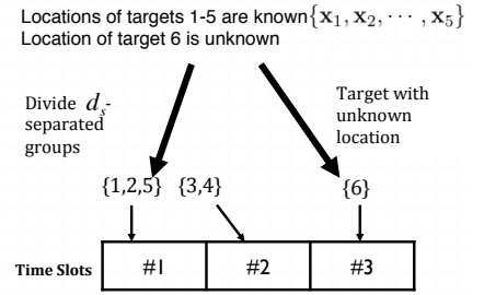
Fig. 8. An example of LBTA to assign time slots
