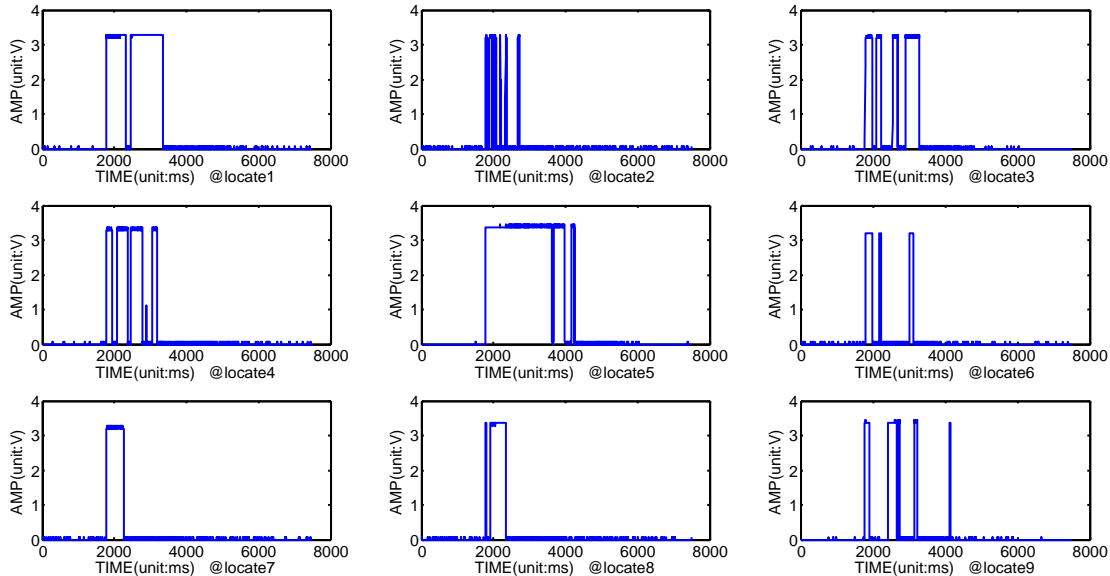
Fig. 19. Signal Captured by 9 receiver
