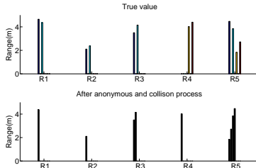
Fig. 13. Range obtained by receivers
