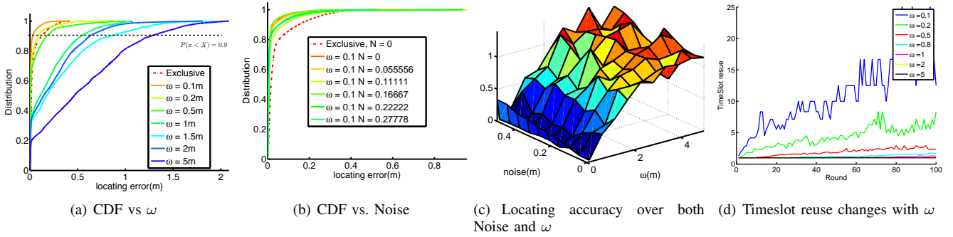
Fig. 15. Robustness and efficiency of chorus locating
