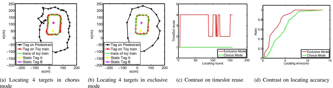
Fig. 20. Evaluating chorus locating in testbed
