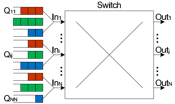
Fig. 1. Switch structure.
