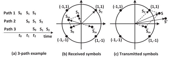
Fig. 6. Refined channel synchronization against the multipath effect.
