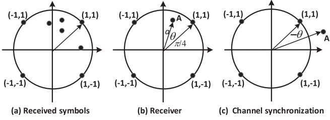
Fig. 5. Basic channel synchronization.
