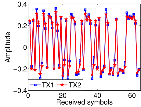
Fig. 4. With channel synchronization.
