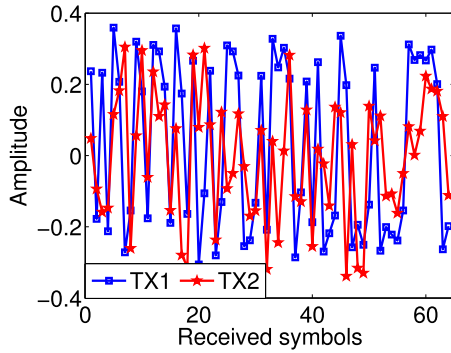
Fig. 3. Without channel synchronization.
