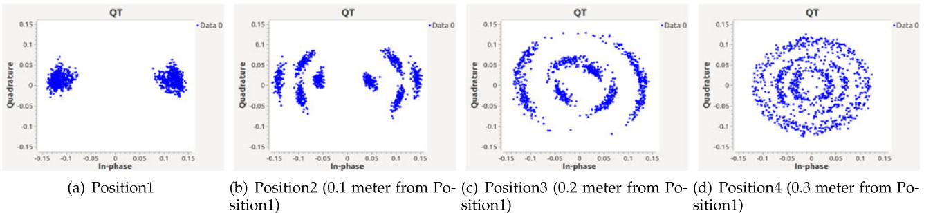
Fig. 12. Jamming signal entanglement.
