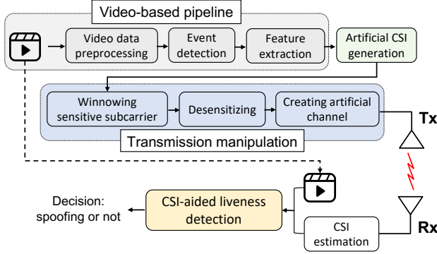
Figure 3: Flow chart of the phantom-CSI attack.
