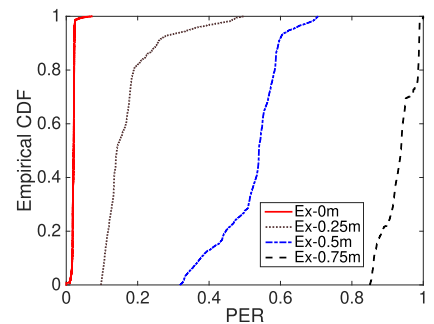
Fig. 9. Eavesdropper's PER.
