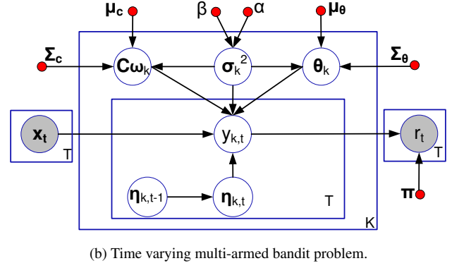
Figure 2: Graphical model representation for bandit problem. Random variable is denoted as a circle. The circle with gray color filled means the corresponding random variable is observed. Red dot represents a hyper parameter.
