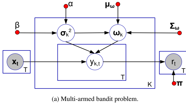
(a) Multi-armed bandit problem.
