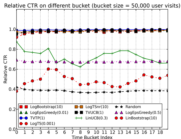
Figure 4: The CTR of KDD CUP 2012 online ads data is given for each time bucket. LogBootstrap , LogTS , LogTSnr , and LogEpsGreedy are bandit algorithms with logistic regression model. LinUCB , LinBootstrap , TVTP , and TVUCB are based on linear regression model.
